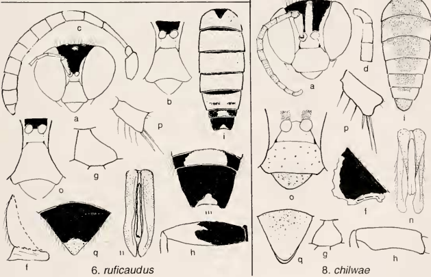
Figs. 5-8. Morphological characters of Bembecinus spp.: 5, parkhuisae ; 6, ruficaudus ; 7, zebratus ; 8, chilwae . Arabic letters a-n indicate male characters (a, face; b, lower face enlarged; c, antenna, front view; d, flagellomeres IX-XI, lateral; e, thoracic pattern; f, outline of left propodeal flange in lateral view; g, second submarginal cell of forewing; h, hindfemur, outer view; i, abdomen with tergal banding, dorsal; k, outline of T-VII; m, terminal terga VI-VII, shape and pattern; n, genitalia, dorsal; n', enlargement of genitalia toward apex; o, lower face except eyes; p, forebasitarsus, lateral outline; q, shape and markings of T-VI; r, markings of female T-III-VI).
